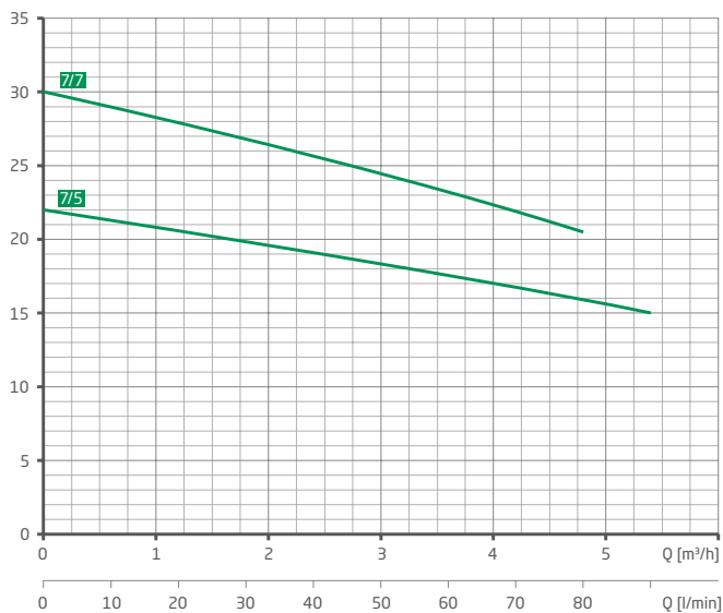
Characteristics VGX 12
