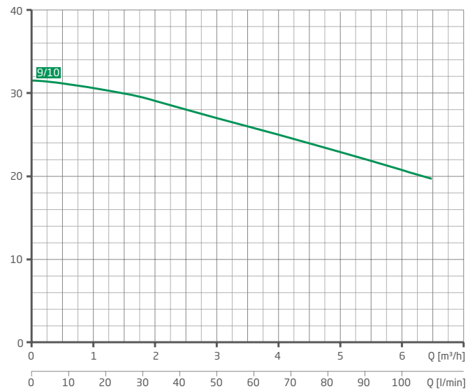
Characteristics VGX 20
